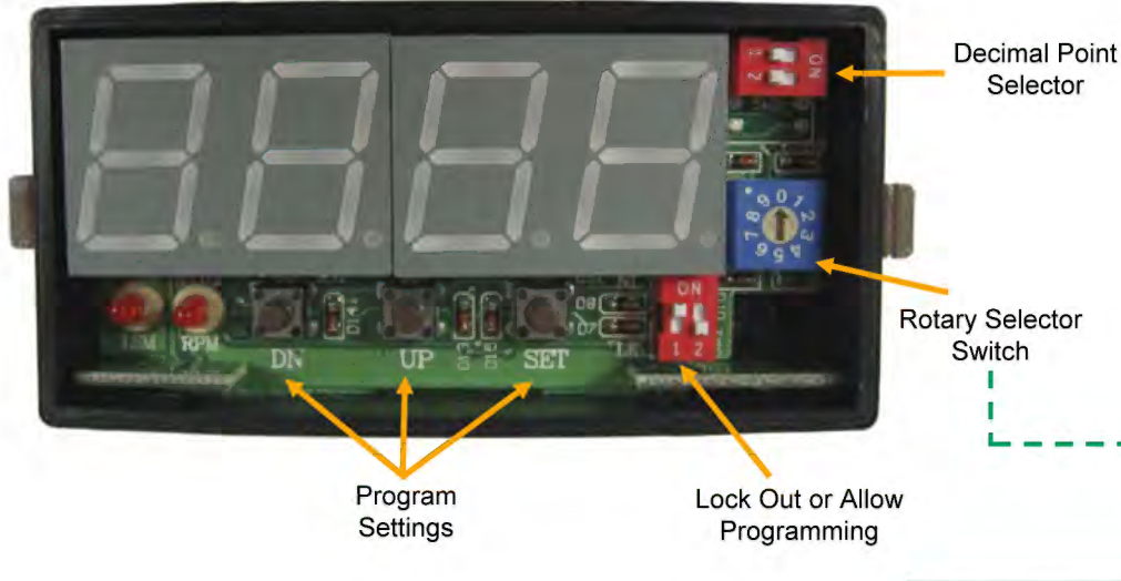
(Tacho with Front Cover Removed)
